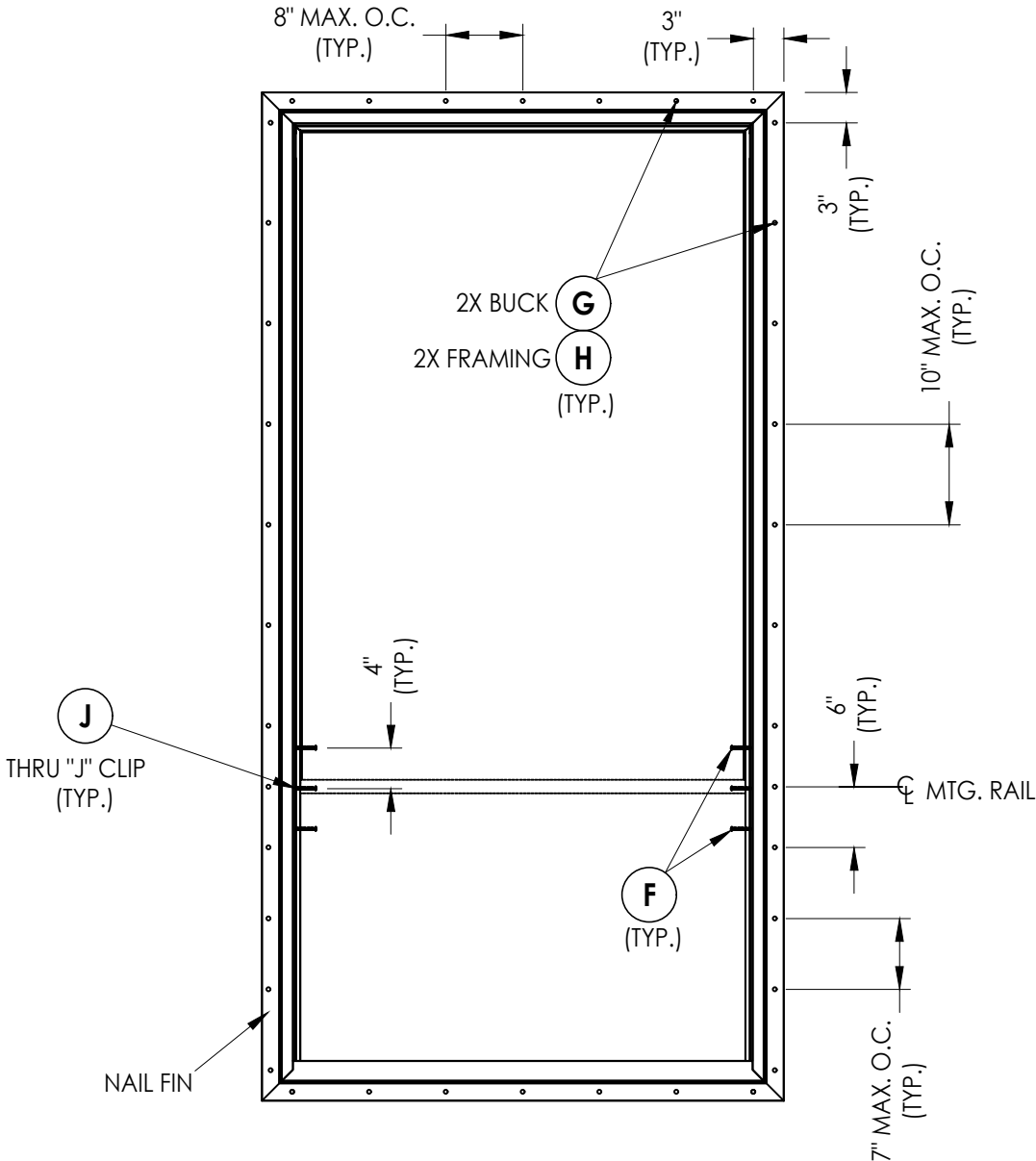
FRAME ANCHORING 48" X 96" MAX. FRAME SIZE
